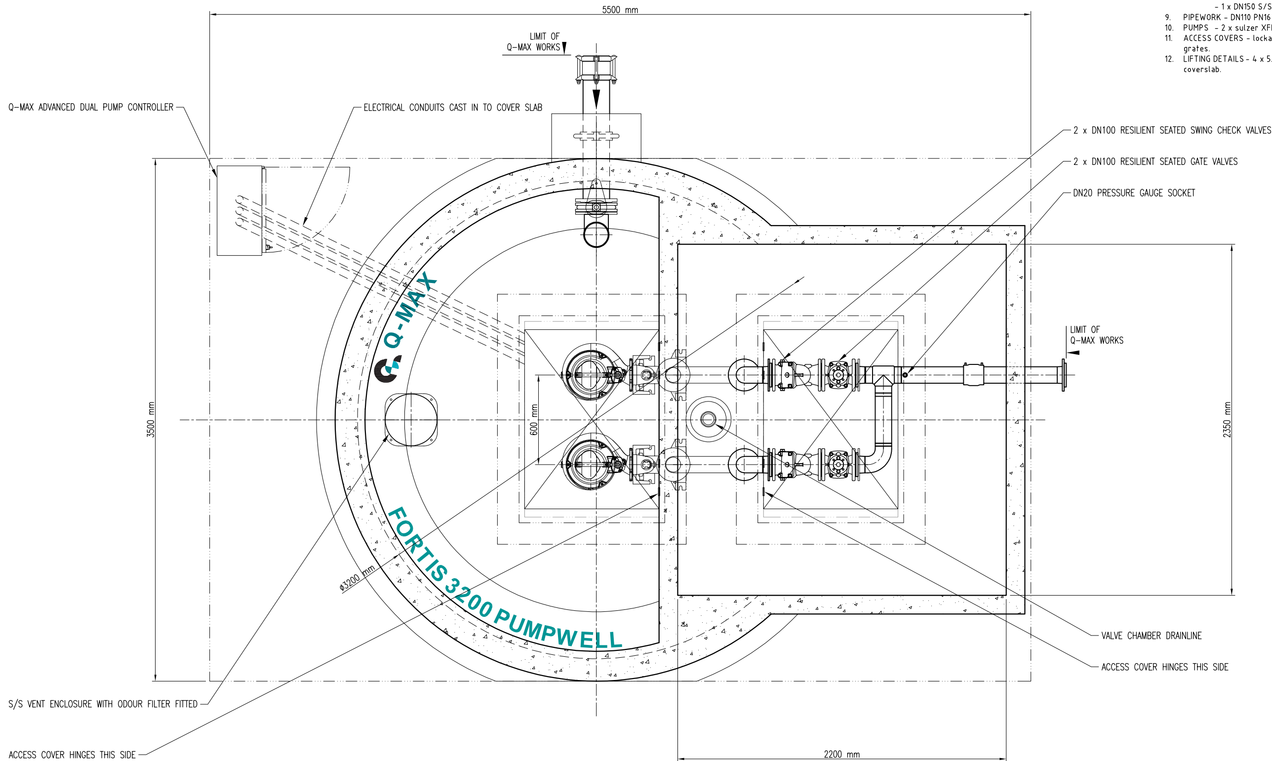
SECTIONAL PLAN VIEW SCALE: 1 : 25 @ A3
